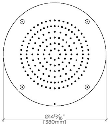
CEILING VIEW SCALE: \frac{1}{2}''=1'-0''
