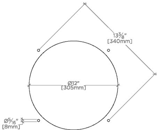
CUTOUT VIEW SCALE: \frac{1}{2}''=1'-0''
