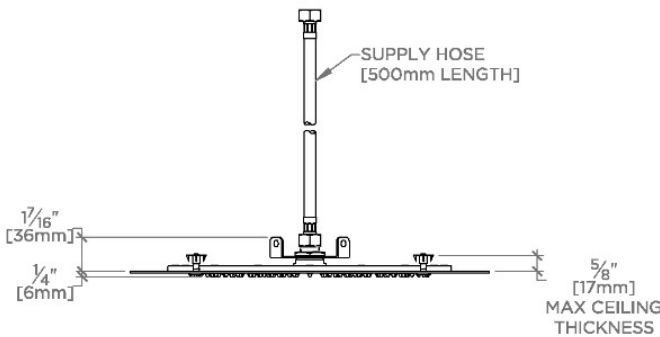
SIDE VIEW SCALE: \frac{1}{2}''=1'-0''
