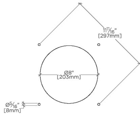
CUTOUT VIEW
