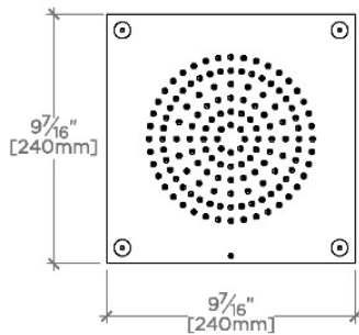
CEILING VIEW
