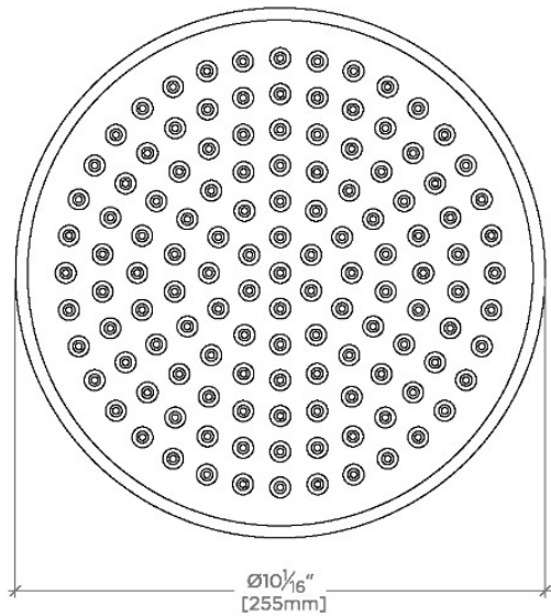
CEILING VIEW
