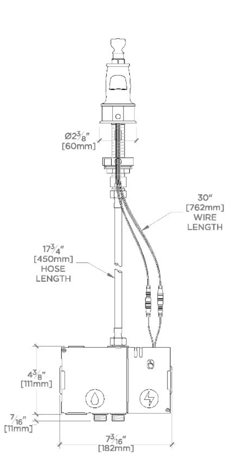
FRONT VIEW
