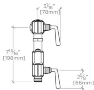
FRONT VIEW SCALE: 1 1/2"=1'-0"
