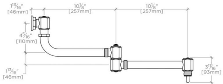
SIDE VIEW SCALE: 1 1/2"=1'-0"
