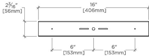
MOUNTING PLATE
