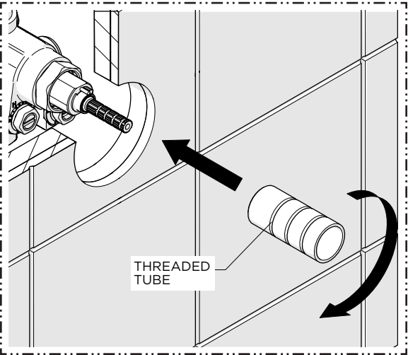
17. Thread the THREADED TUBE back into the RETAINING NUT until snug.
