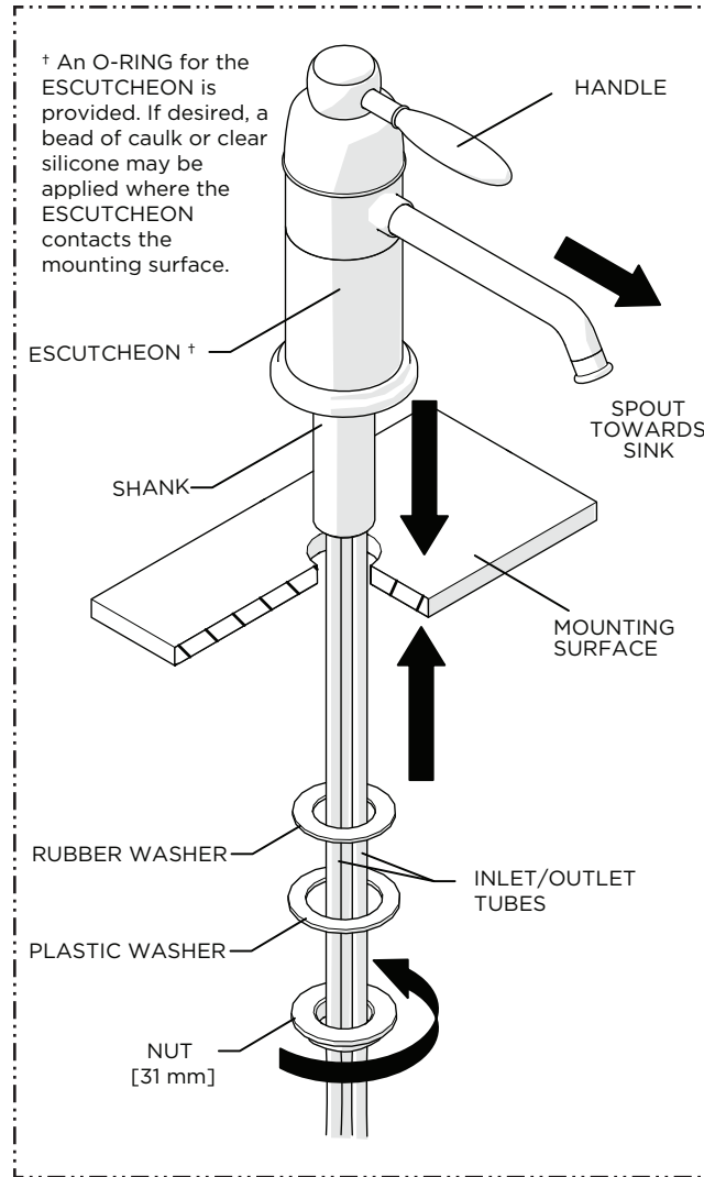
STYLE No. UNWD10 Universal Traditional One Hole Instant Hot and Filtered Cold Water Dispenser with Metal Lever Handle
