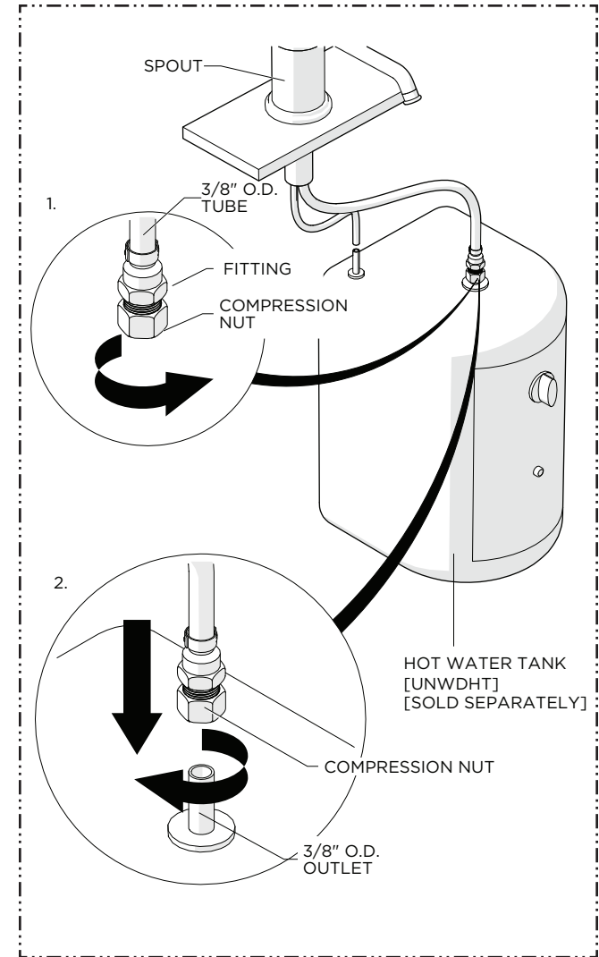
STYLE No. UNWD10 Universal Traditional One Hole Instant Hot and Filtered Cold Water Dispenser with Metal Lever Handle
