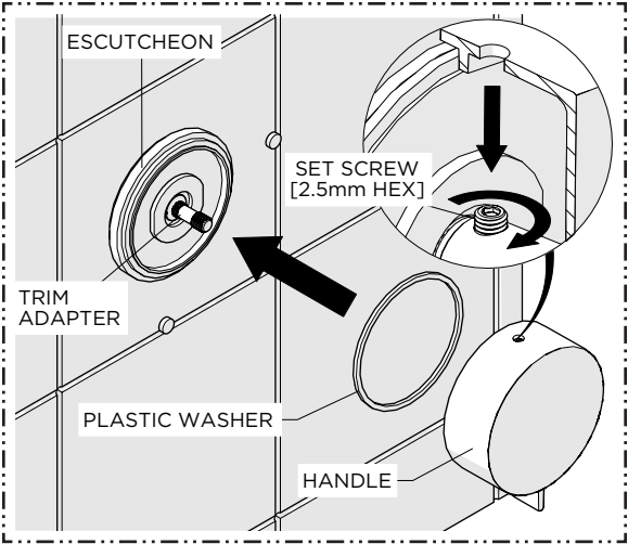
16. Slide the PLASTIC WASHER onto the ESCUTCHEON then place the HANDLE onto the TRIM ADAPTER. Ensure the HANDLE is fully seated and properly aligned with the PINS then thread and securely tighten the SET SCREW.
