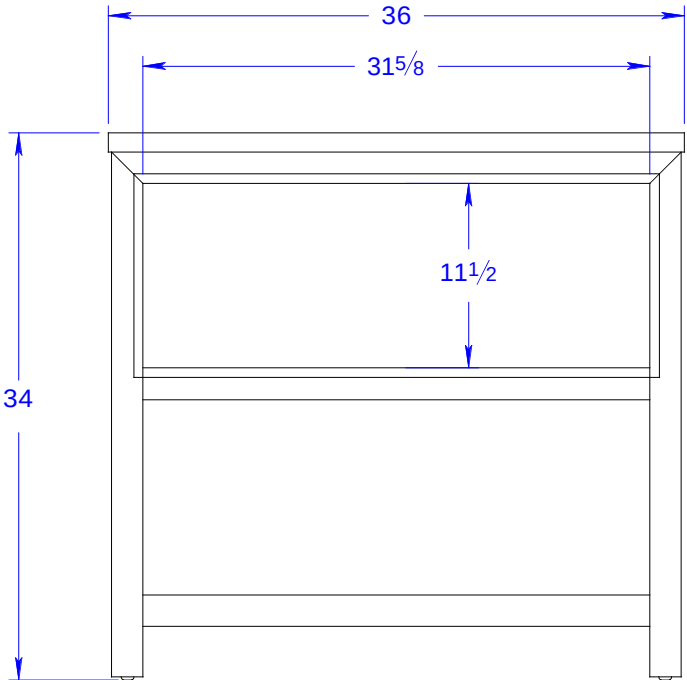
BACK VIEW
