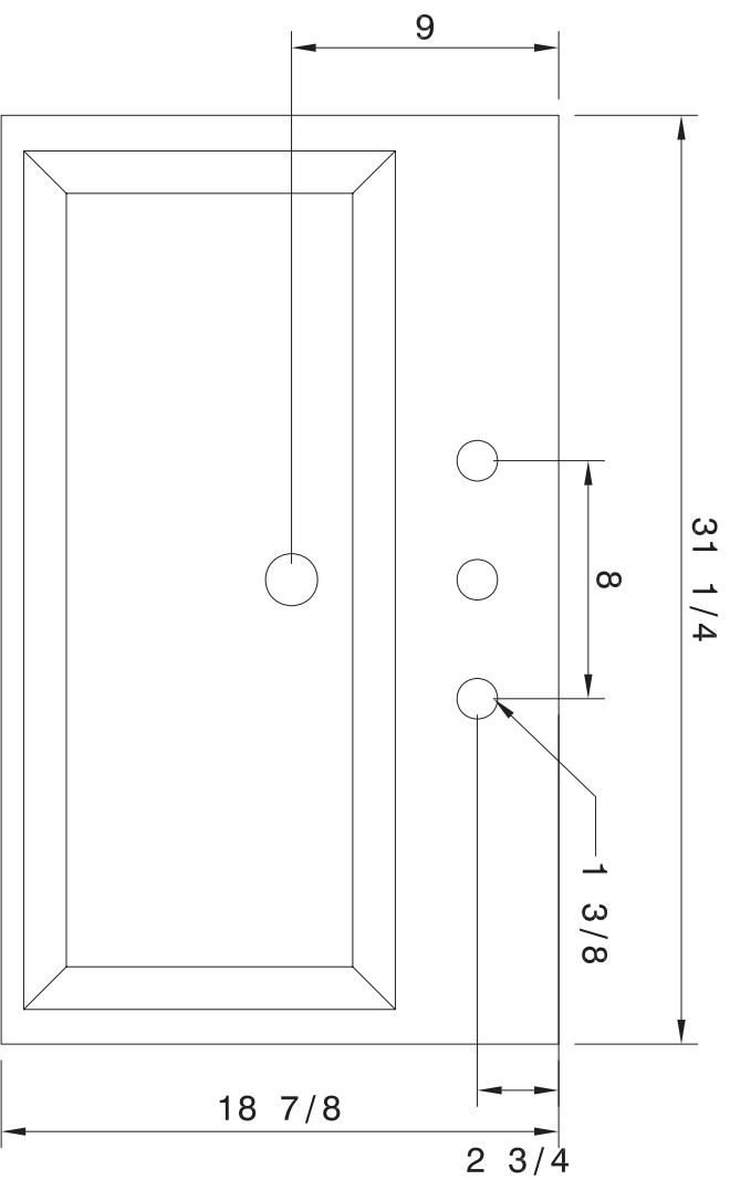
TOP VIEW SINK
