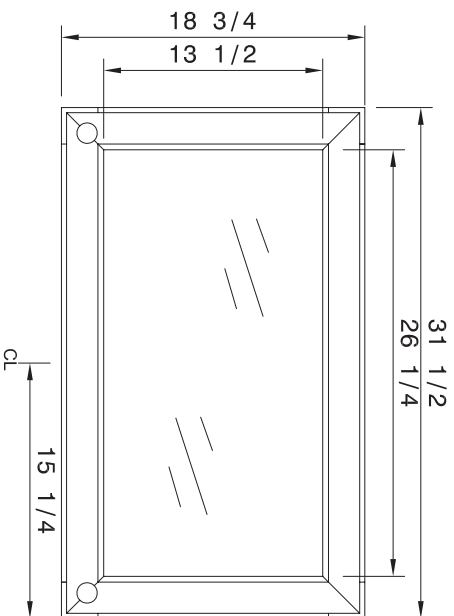
TOP VIEW CONSOLE
