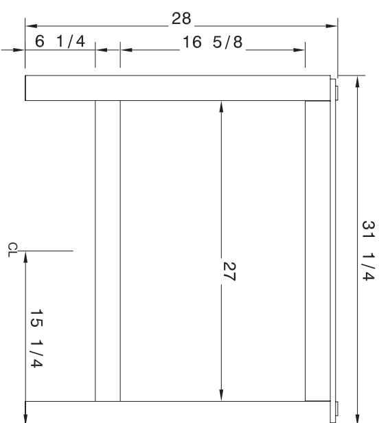
BACK VIEW
