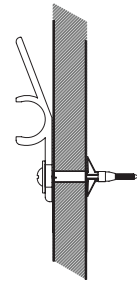
DRYWALL WITHOUT AVAILABLE WOOD STUD Plug with wall anchor
