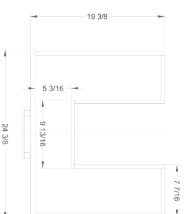
DRAWER A TOP VIEW
