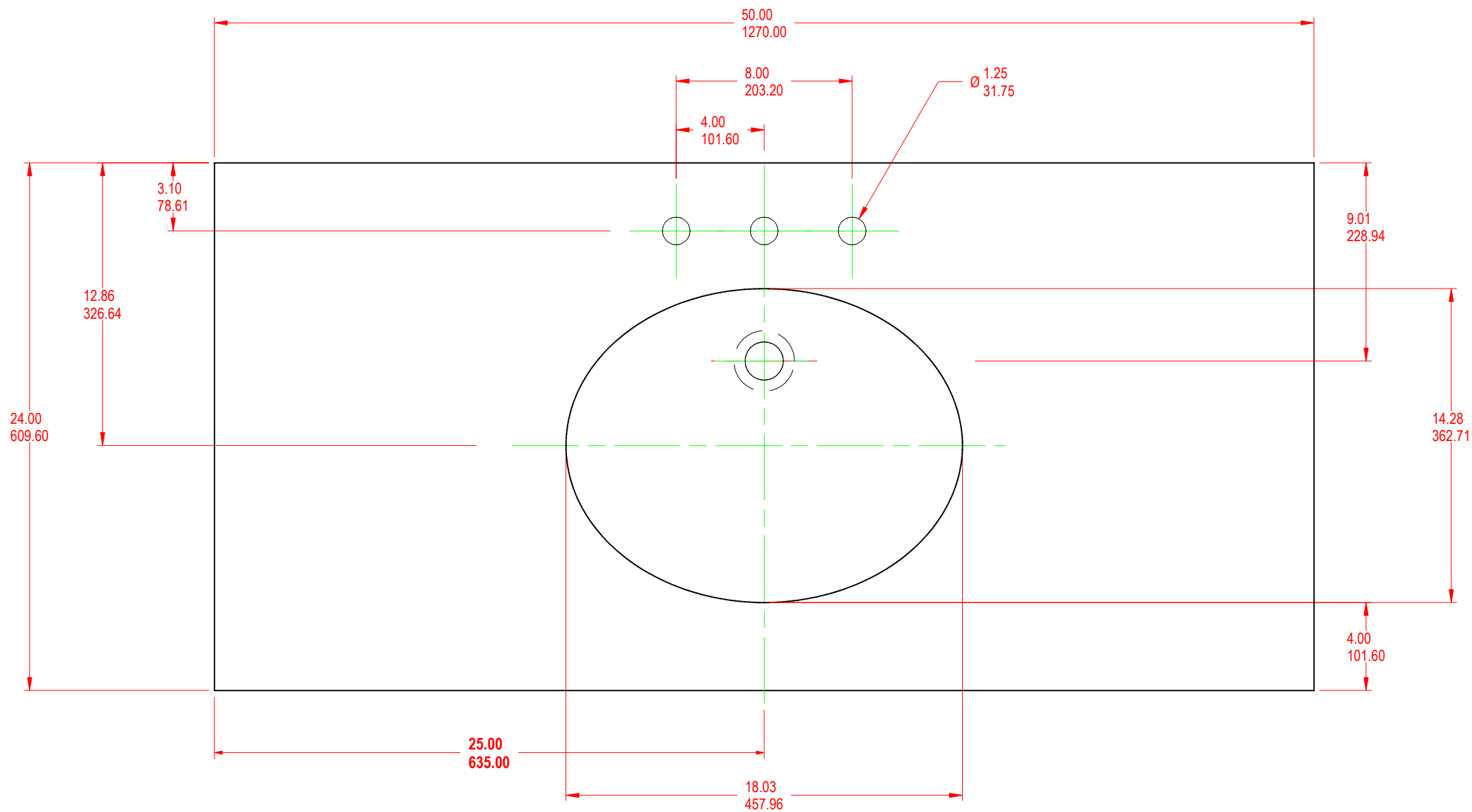
PLAN VIEW
