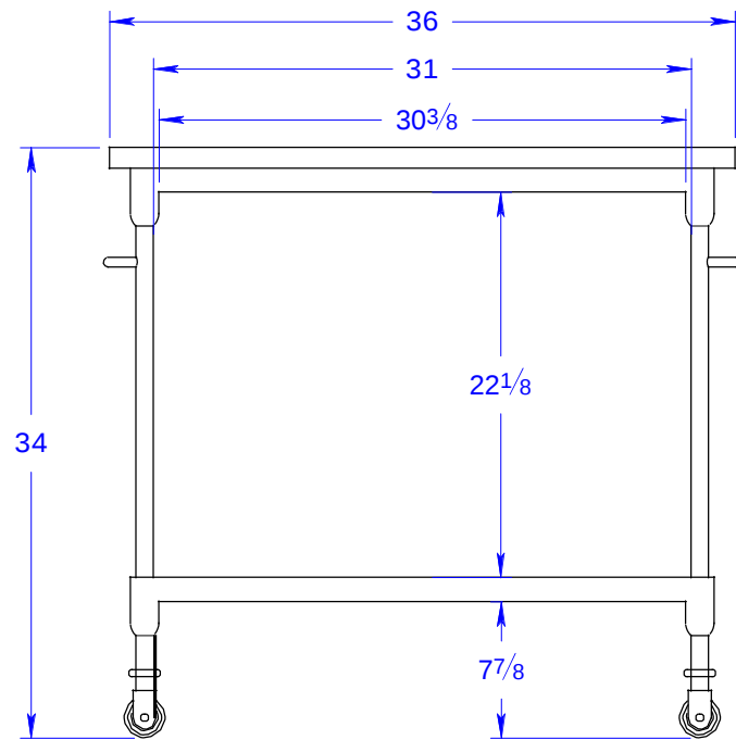
BACK VIEW
