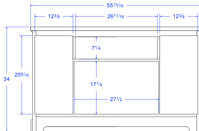
BACK VIEW
